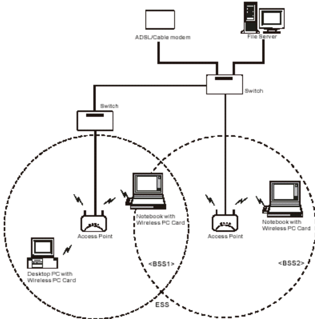
Figure 1-3 Seamless Roaming
